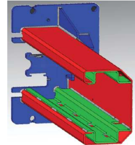
Internally reinforced colomn structure.
