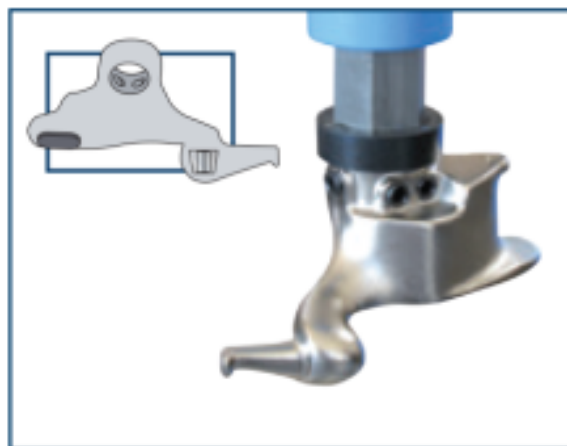
TOOL WITH INTEGRATED PROTECTION FOR ALLOY RIMS
